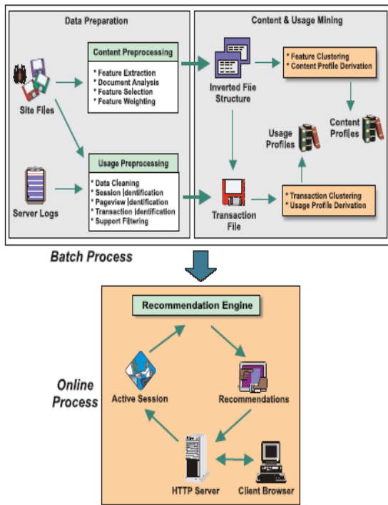
Figure 1. A general framework for Web personalization based on usage and content mining. The data preparation and mining tasks are performed offline resulting in a uniform representation for both usage and content profiles. The real-time recommendation engine uses these profiles and the current active user session to provide recommendations.
